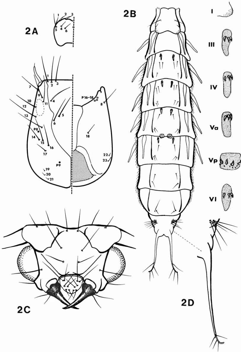
Fig. 2. Hudsonema flaminii (Navás), larva and pupa. A, Larva, head and labrum (detached) setal pattern, left half dorsal, right half ventral. B, Pupa, abdomen, dorsal, hook plates enlarged. C, Pupa, head, frontal. D, Pupa, right anal process, dorsal.
